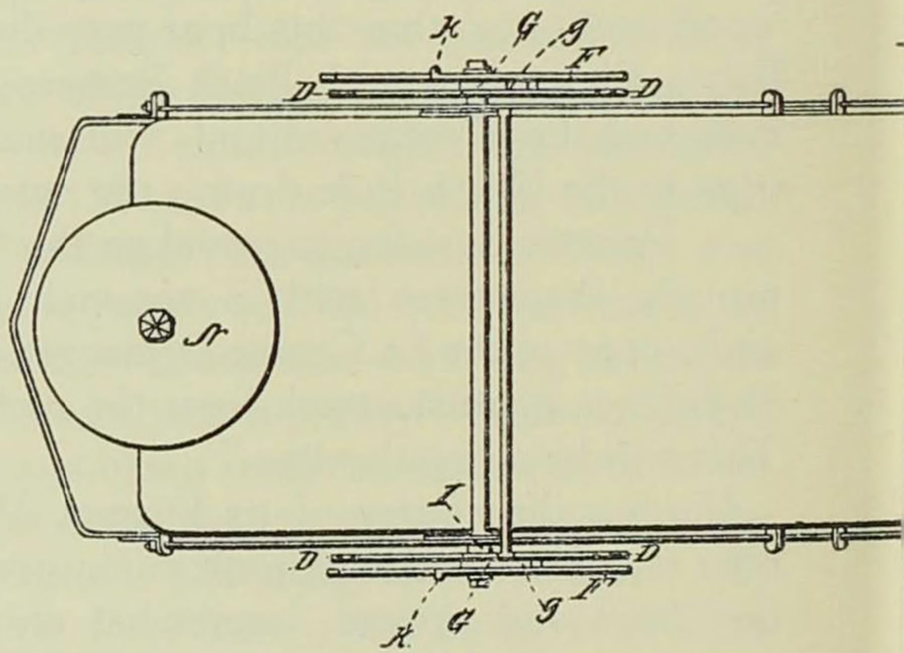
SIDE ELEVATION AND UNDERSIDE VIEW OF WIARD'S ICE BOAT AS PATENTED ON JANUARY 24, 1860
