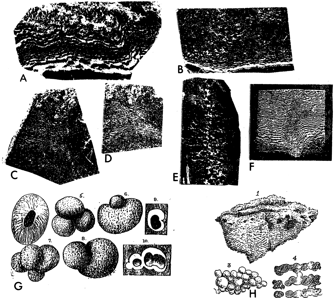
A-D, Eozoon canadense collected recently (1993), sliced and reproduced by means of placing the slice on a Xerox machine, all x1. E, Archaeospherina slab reproduces by Xerox machine, x1/2. F, Eozoon reproduced from 19th century literature, x1/2. G, "Buds" of Eozoon or Archaeospherina from 19th century literature, x3. H, Eozoon and Archaeospherina from wood cut of original Eozoon paper, 1868.
