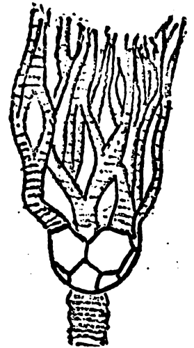
CYATHOCRINITES
