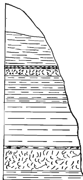
FIG. 3—Vertical section in clay pit at Redfield.
