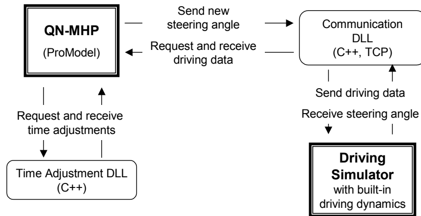
Figure 2. Block diagram of the interface between QN-MHP and the driving simulator
